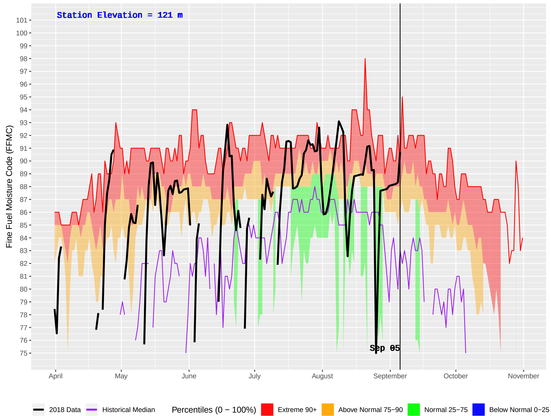
BOWSER (56) : Historical (1985–2016) and Current (2018) Daily Fine Fuel Moisture Code (FFMC)
