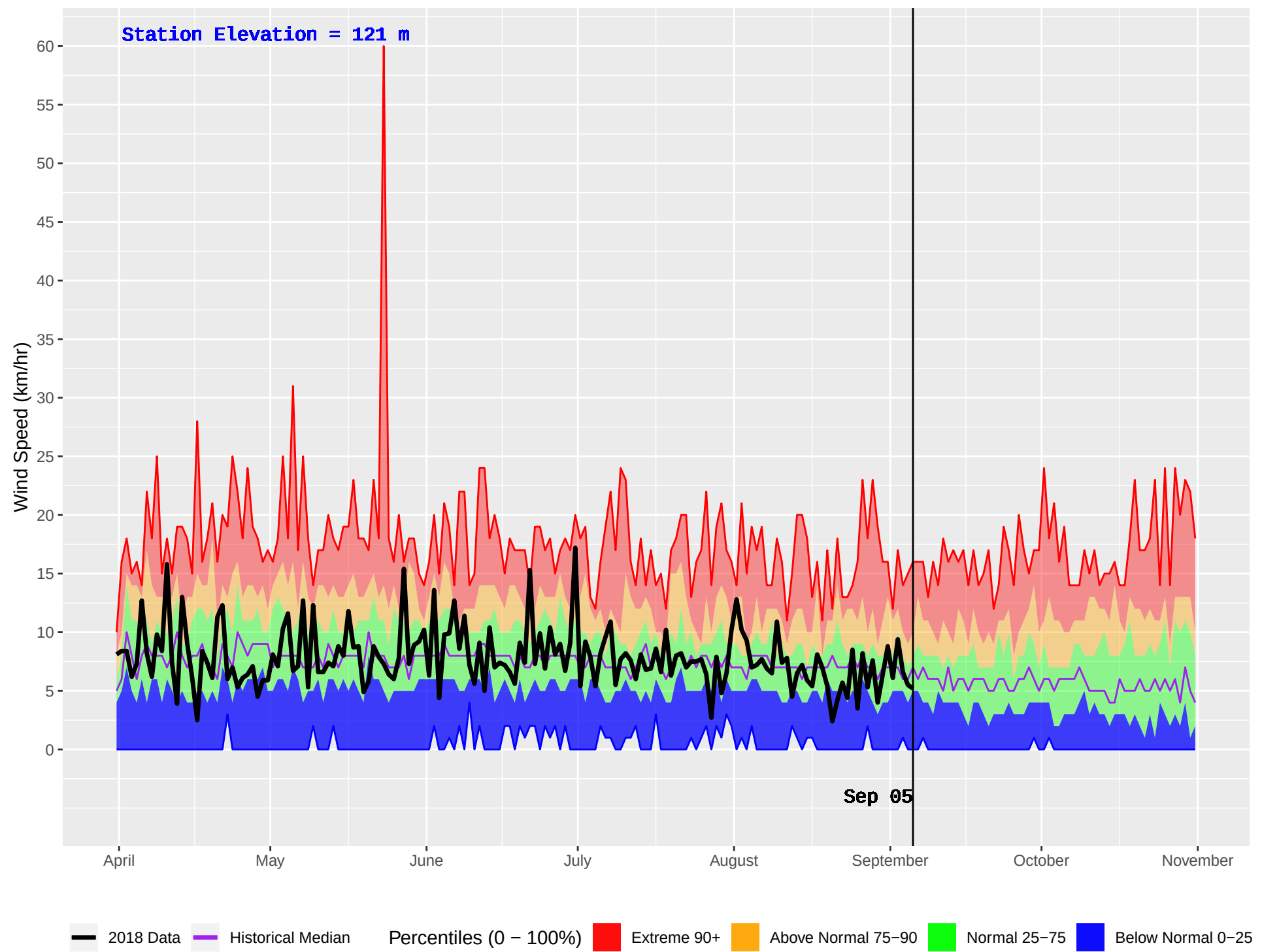
BOWSER (56) : Historical (1985–2016) and Current (2018) Daily Wind Speed
