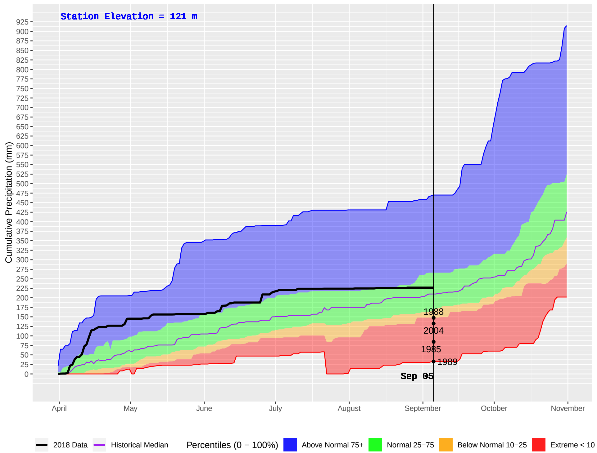
BOWSER (56) : Historical (1985–2016) and Current (2018) Daily Cumulative Precipitation
