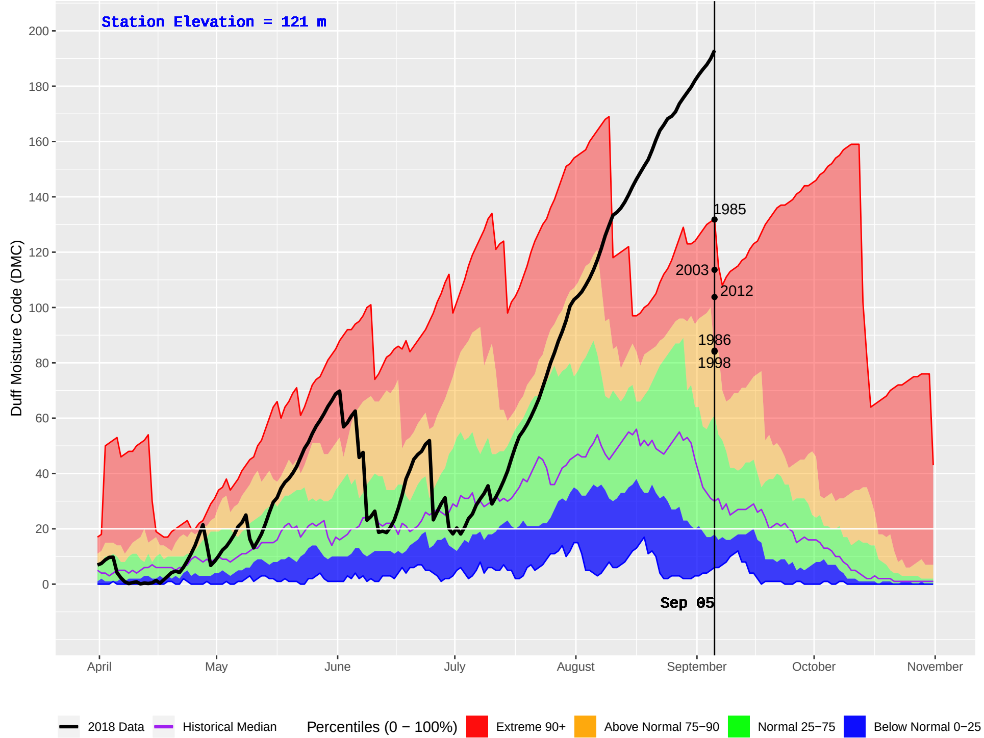
BOWSER (56) : Historical (1985–2016) and Current (2018) Daily Duff Moisture Code (DMC)
