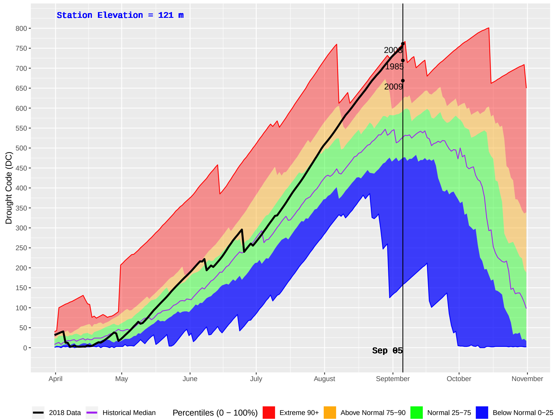
BOWSER (56) : Historical (1985–2016) and Current (2018) Daily Drought Code (DC)
