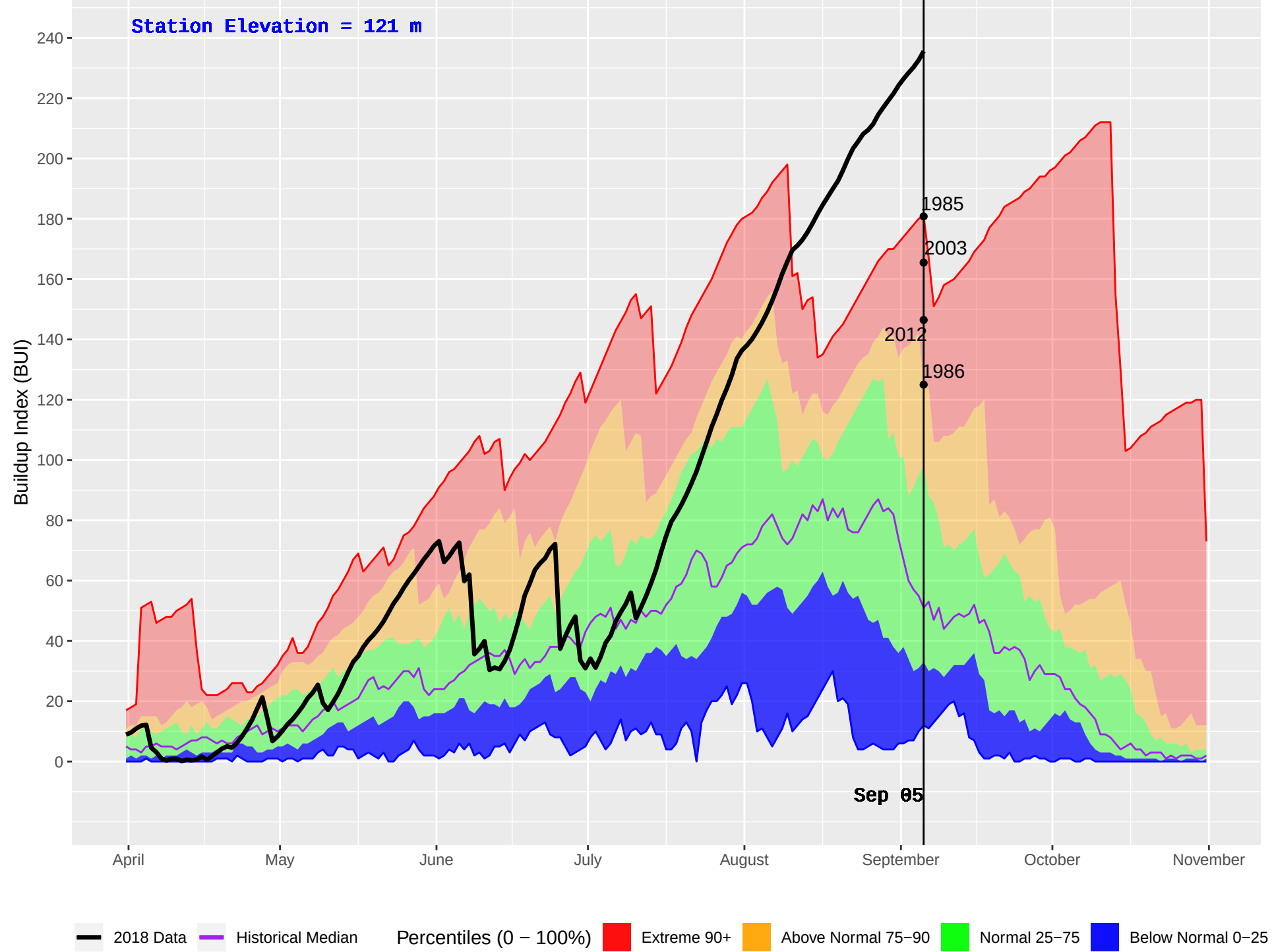
BOWSER (56) : Historical (1985–2016) and Current (2018) Daily Buildup Index (BUI)
