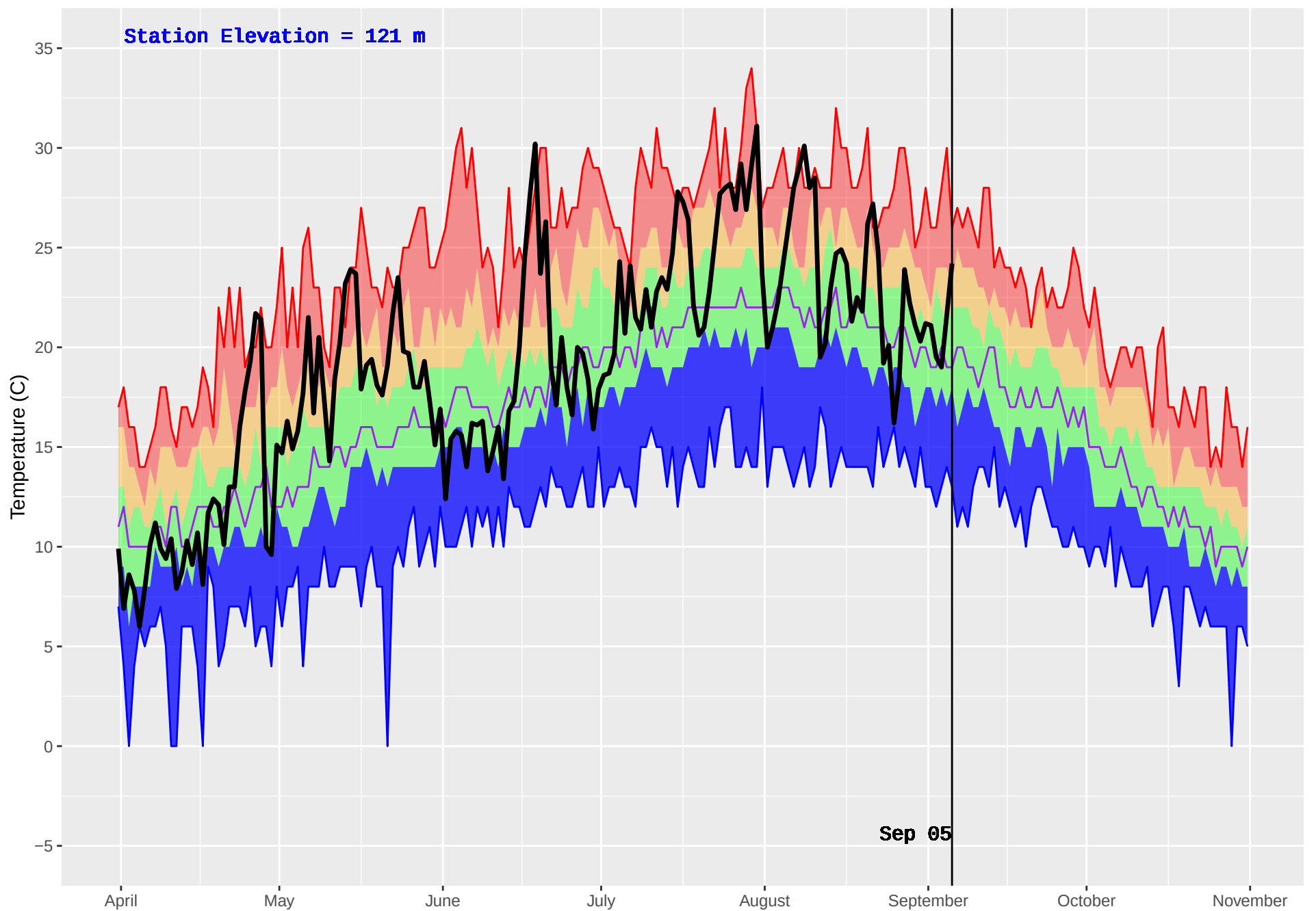
BOWSER (56) : Historical (1985–2016) and Current (2018) Daily Temperature
