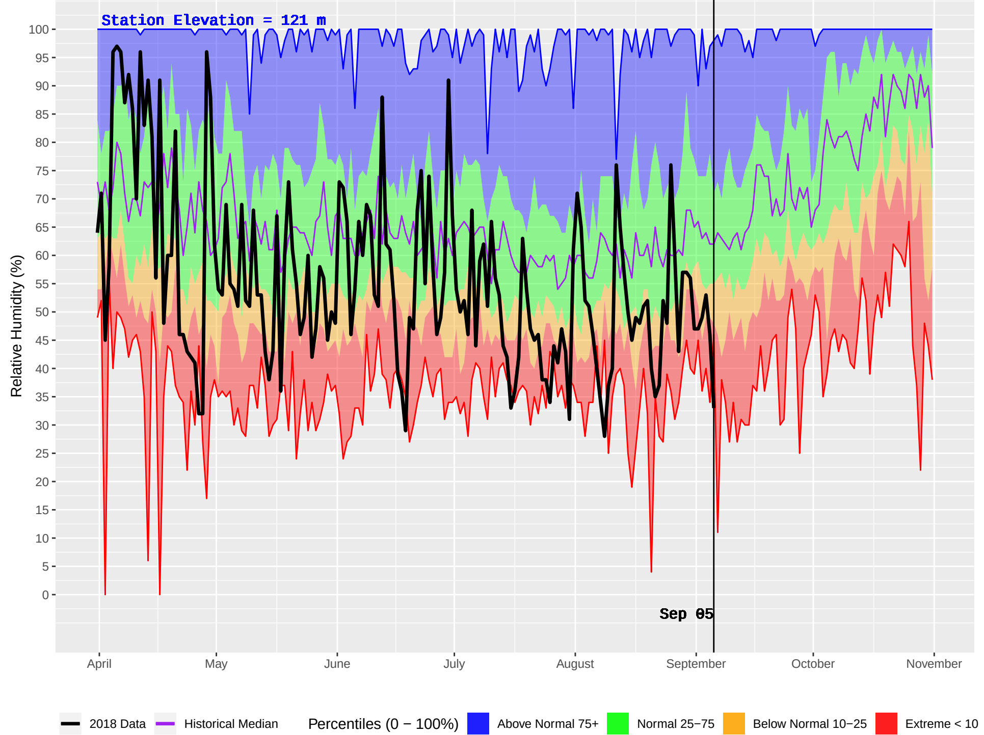
BOWSER (56) : Historical (1985–2016) and Current (2018) Daily Relative Humidity
